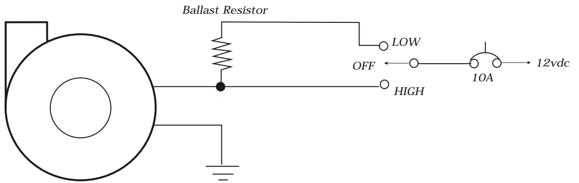
Wiring Diagram for 82 VW Rabbit Blower Motor
